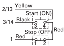
Figure B START/STOP Selector Switch
