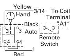
Figure C 3-Position Selector Switch
