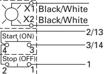
Figure F START/STOP with Pilot Light Connect to "A1" and "A2" Terminals
